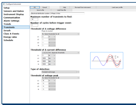
Configure transient voltage peaks and current waveforms.
