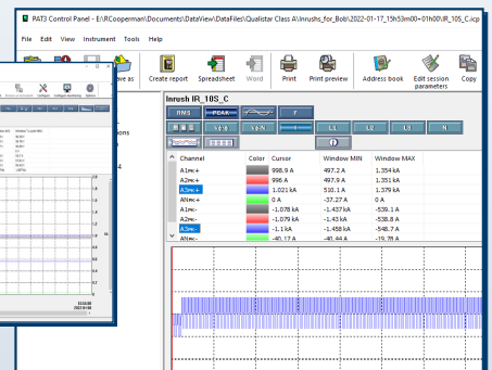
Display InRush peak.
