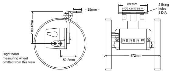
Product Dimensions 2300
