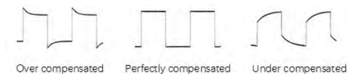
Figure 5.6 Probe Compensation
