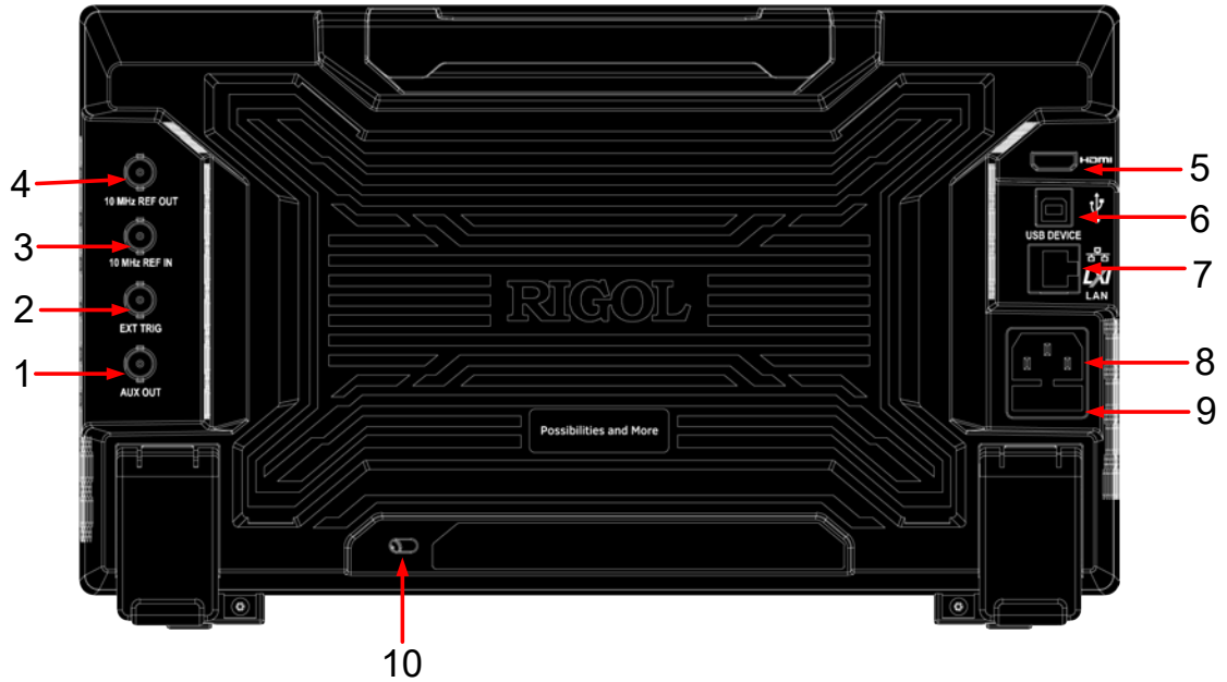
Figure 4.3 Rear Panel
