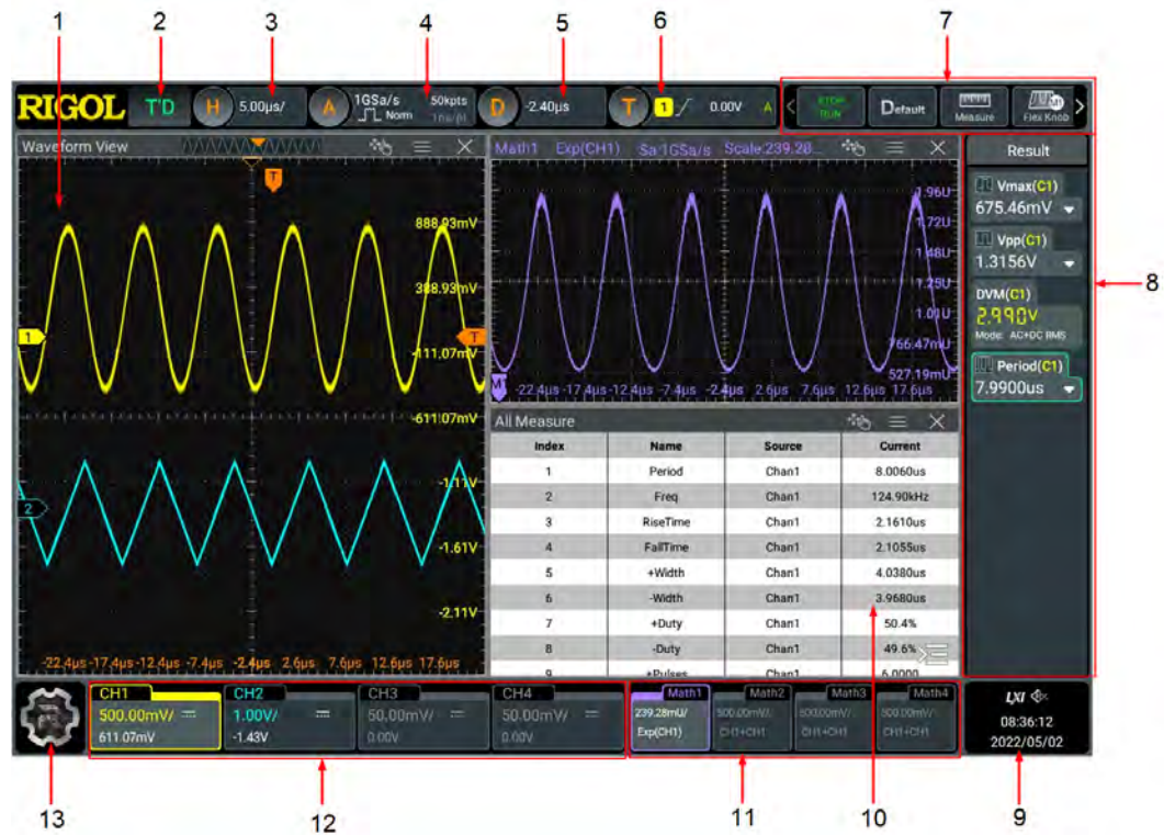
Figure 4.4 User Interface
