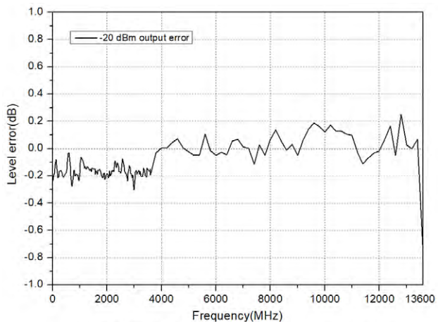
Measured at -20 dBm, level error vs frequency
