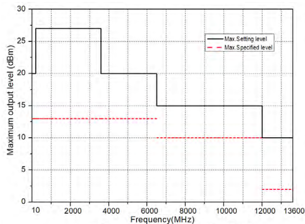
Maximum output level vs frequency
