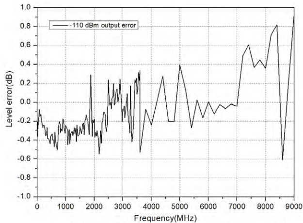
Measured at -110 dBm, level error vs frequency
