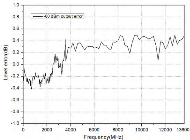
Measured at -60 dBm, level error vs frequency
