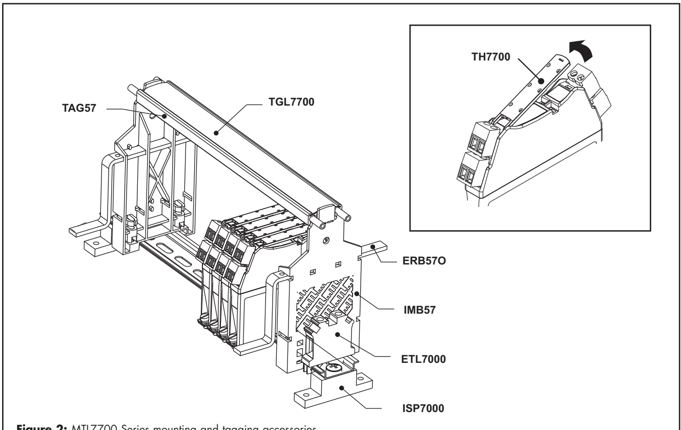
Figure 2: MTL7700 Series mounting and tagging accessories
