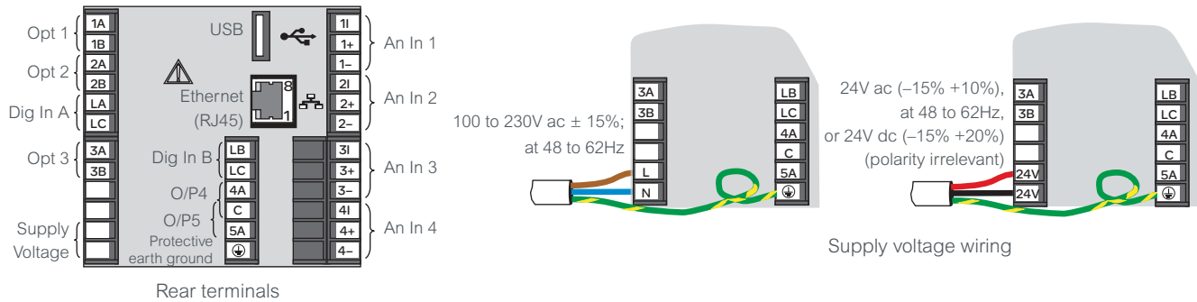
Rear terminals
