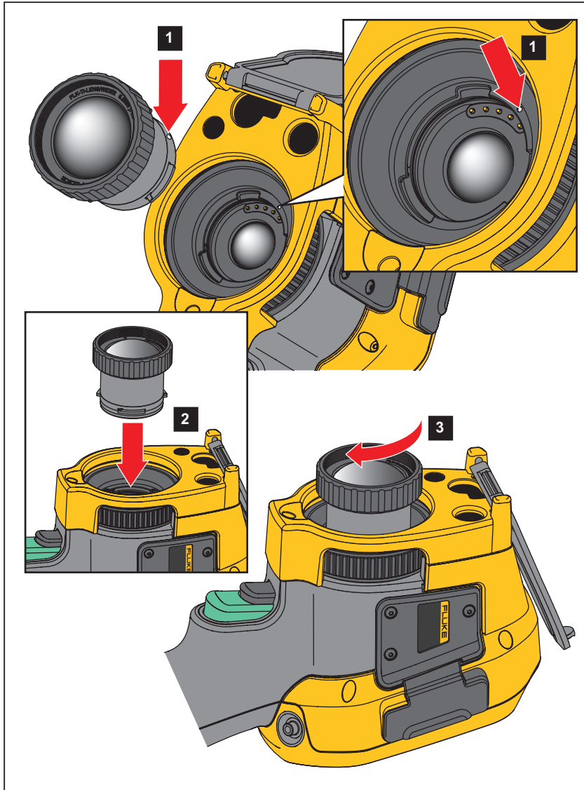
Figure 1. Optional Lens Installation
