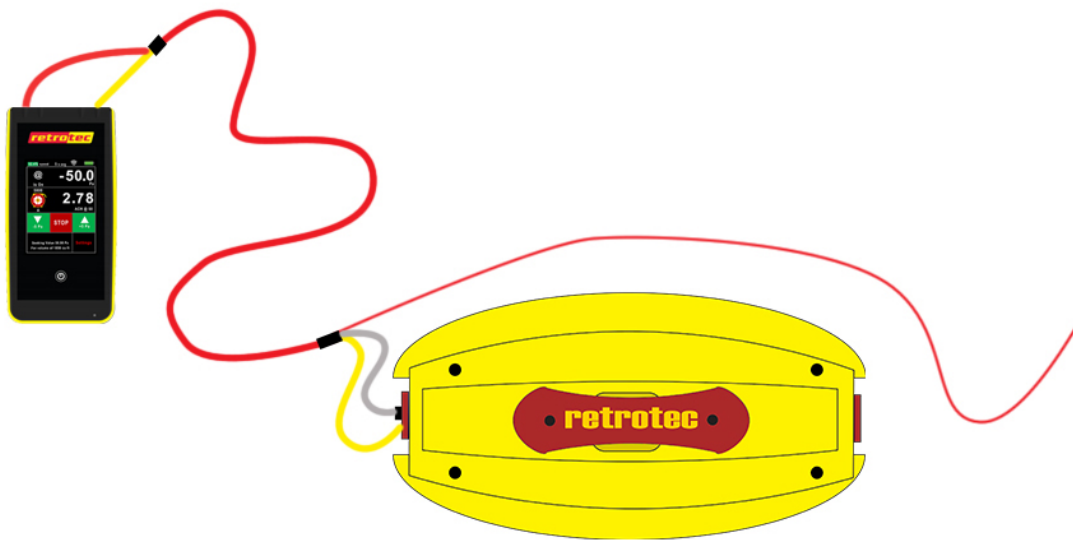
Figure 15: DM32 to fan connection.
