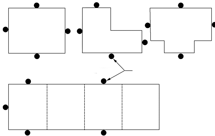
Figure 14 typically recommended locations for exterior pressure pickups
